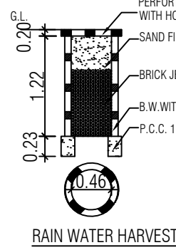
RAIN WATER HARVEST
