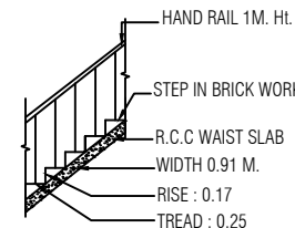
STAIR DETAIL
