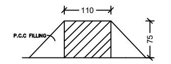
DWARF WALL SECTION
