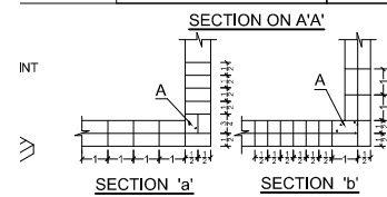
TYPICAL DETAILS OF PROVIDING VERTICAL STEEL BARS IN BRICK MASONRY
