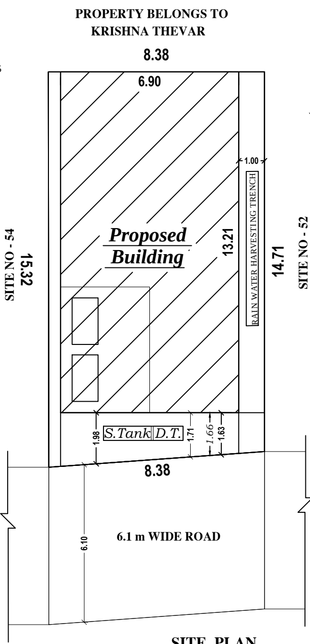
SITE PLAN
