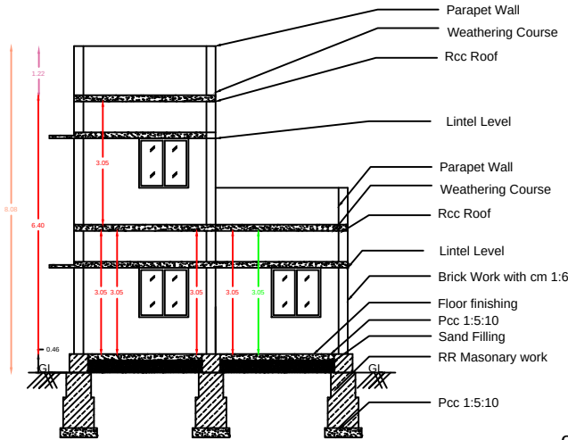
SECTION ON-"AB"
