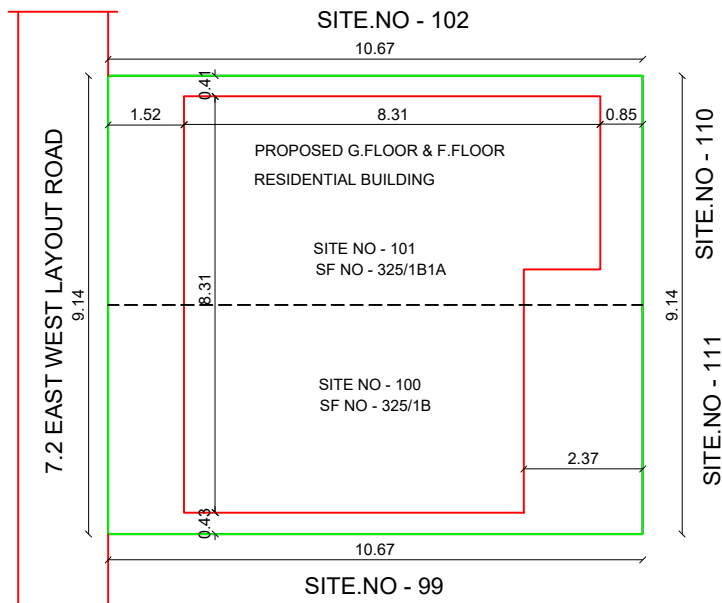
SITE PLAN
