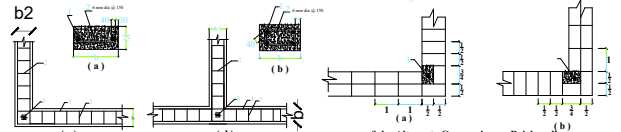
a & b. Alternate Courses in one Brick wall 1 : one Brick Length 1/2 : Half Brick Length 1/4 : Quarter of a Brick Length 3/4 : Three Quarters of a Brick Length 3. Vertical Reinforcement bars with Concrete/Mortar Filling in Pocket of M20 Grade (1:1 1/2 :3)
