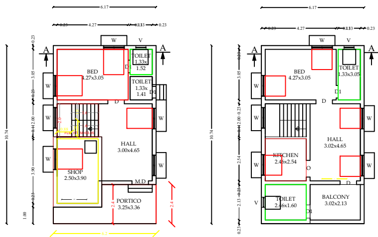
PROPOSED COMMERCIAL(ALTERATION) GROUND FLOOR & EXISTING GROUND FLOOR
