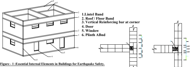
Figure - 1 : Essential Internal Elements in Buildings for Earthquake Safety.
