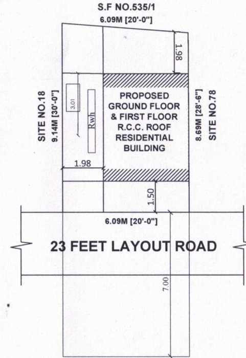
SITE PLAN SCALE = 1:100
