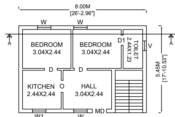
EXISTING GROUND FLOOR
