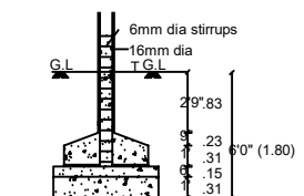
COLUMN FOUNDATION DETAIL
