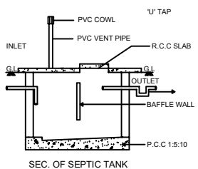
SEC. OF SEPTIC TANK
