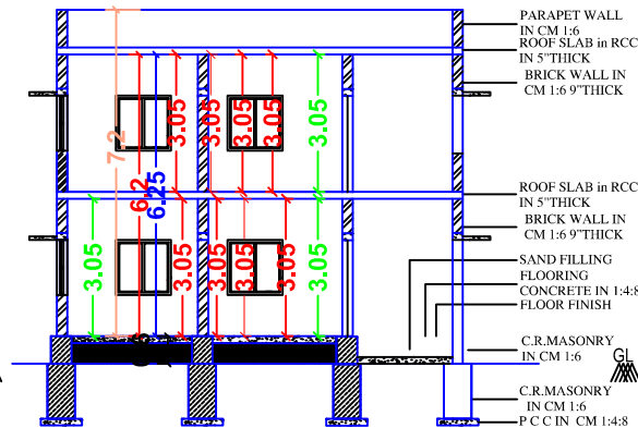
CROSS SECTION
