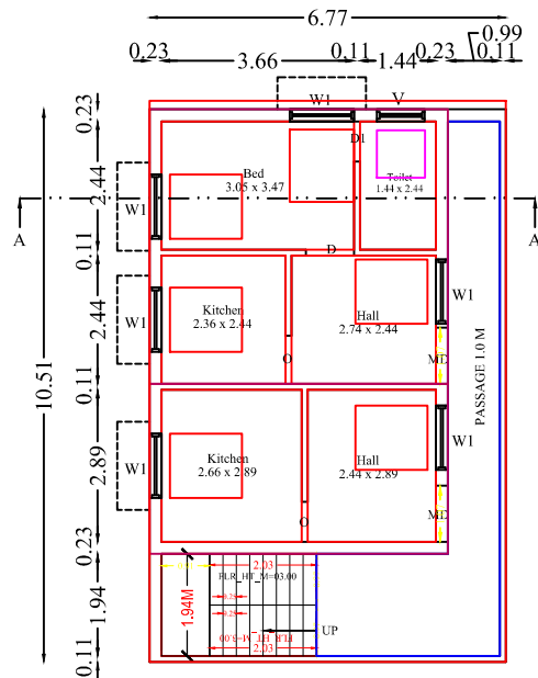
Ex.First Floor Plan Floor-01
