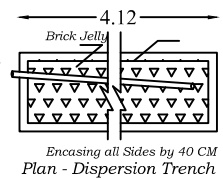
Plan - Dispersion Trench
