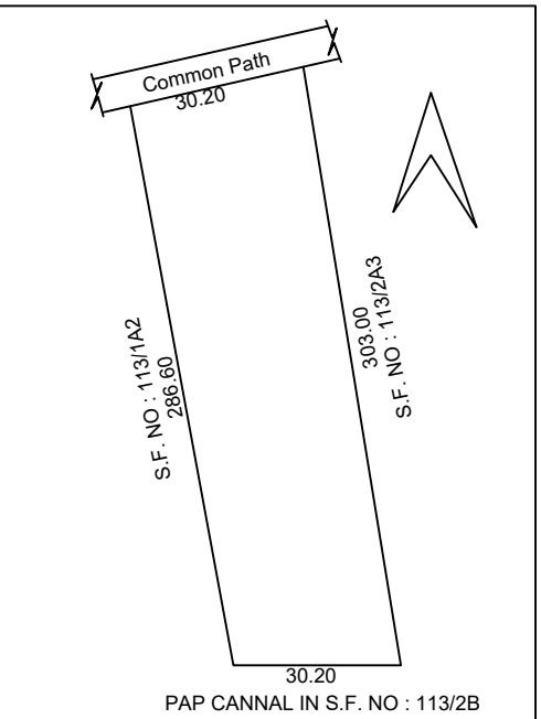
SITE PLAN [NTS]
