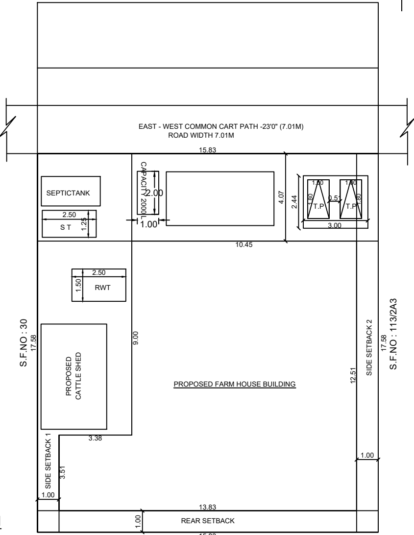
SITE PLAN [MEANT FOR CONSTRUCTION]
