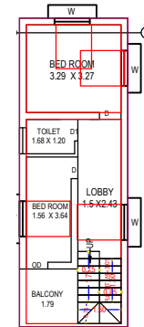
PROPOSED FIRST FLOOR PLAN
