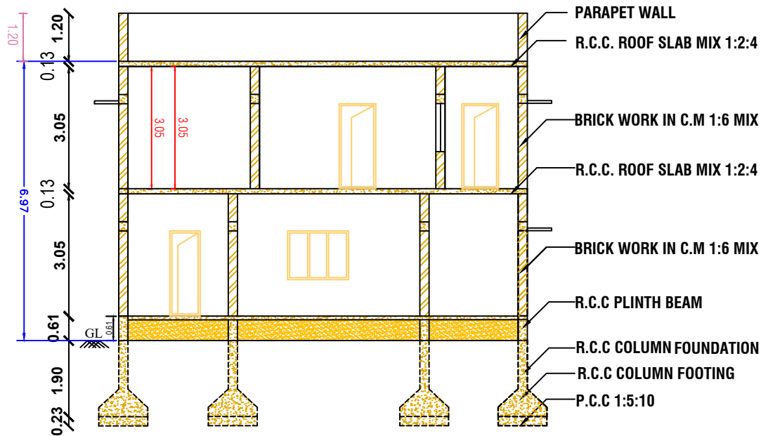
CROSS SECTION AT A-A
