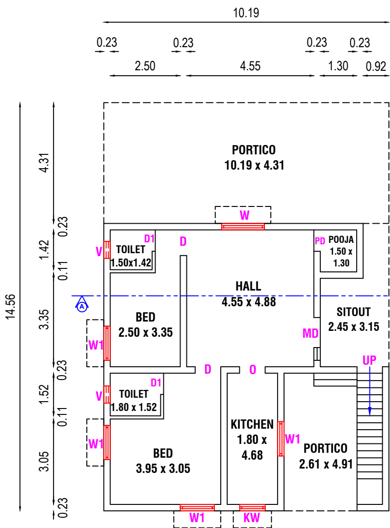
IND ADD. PROPOSED LOOR PLAN
