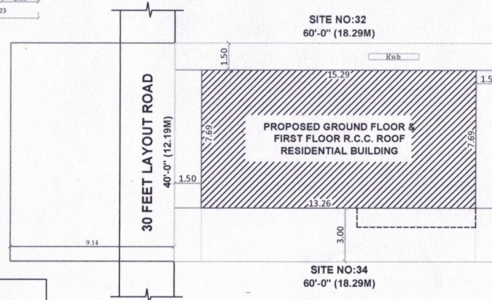
SITE PLAN
