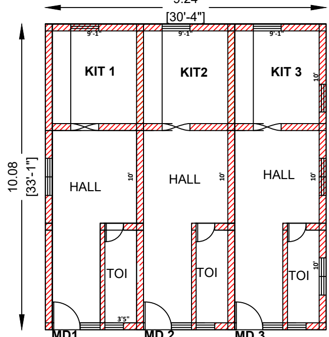
PROPOSED GROUND FLOOR PLAN NO. OF DWELLING UNITS : 3 ( THREE )
