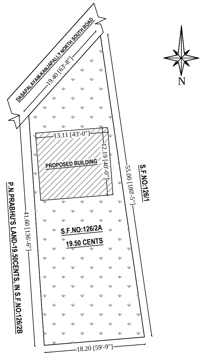
SITE PLAN
