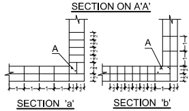
SECTION ON A-A' TYPICAL DETAILS OF PROVIDING VERTICAL STEEL BARS IN BRICK MASONRY A : VERTICAL REINFORCEMENT BARS WITH M20 GRADE CONCRETE a & b : ALTERNATE COURSES IN 1 BRICK WALL 1 : ONE BRICK LENGTH 1/2 : HALF BRICK LENGTH 3/4 : THREE QUARTERS BRICK LENGTH
