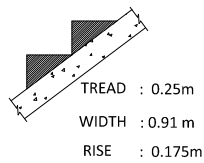
STAIRCASE DETAIL:
