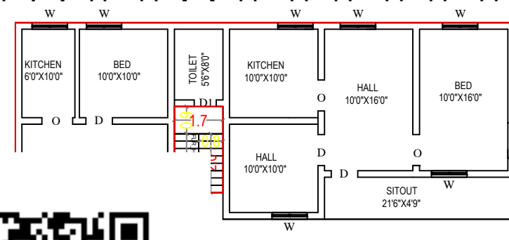
IG GROUND FLOOR PLAN
