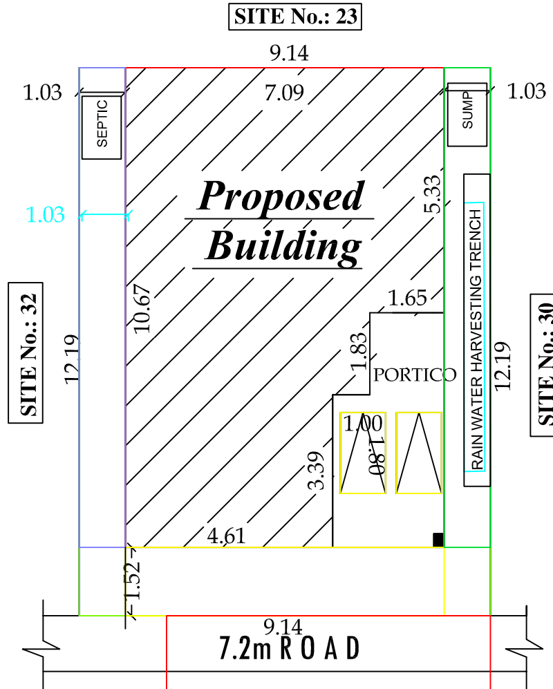
SITE PLAN
