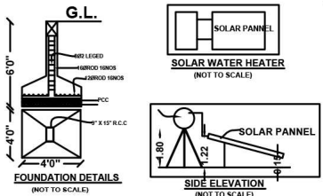
FOUNDATION DETAILS
