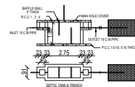
SEPTIC TANK & TRENCH
