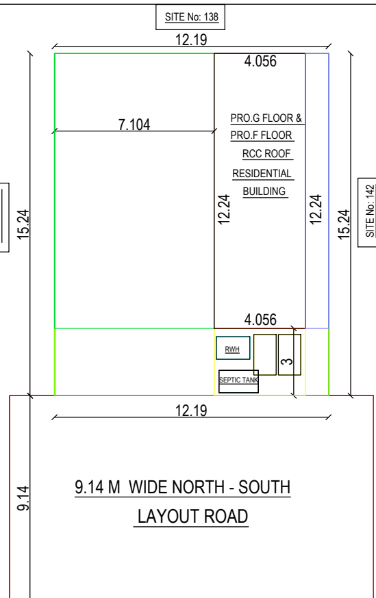
SITE PLAN
