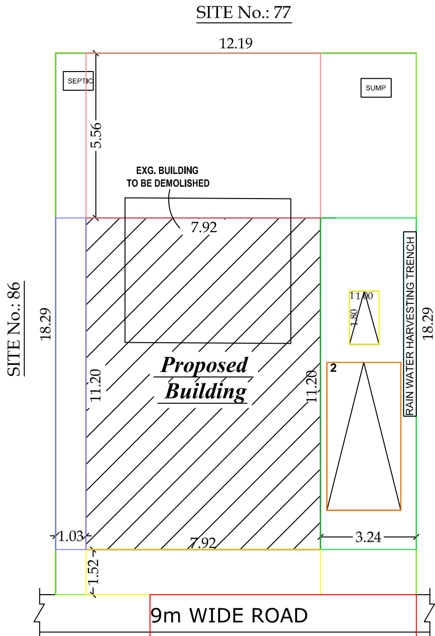
SITE PLAN
