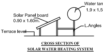
CROSS SECTION OF SOLAR WATER HEATING SYSTEM
