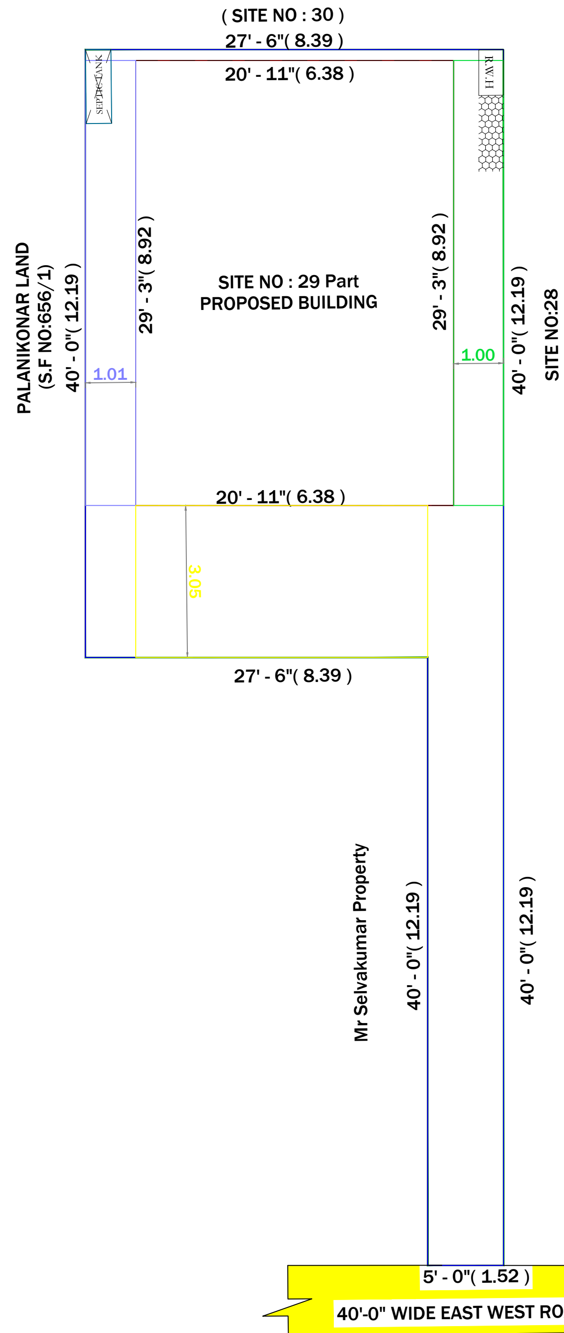
SITE PLAN
