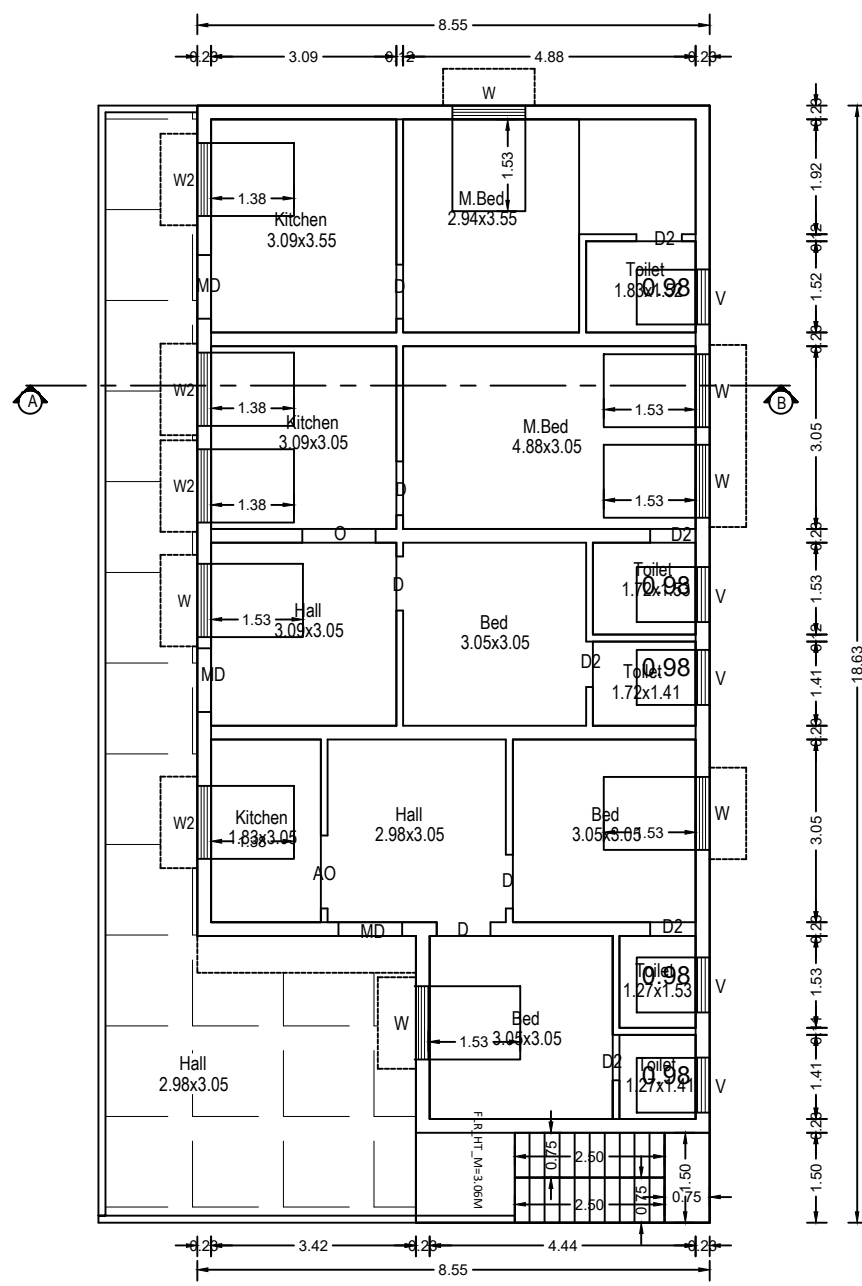
Plan Scale 1:100 Pro. First floor
