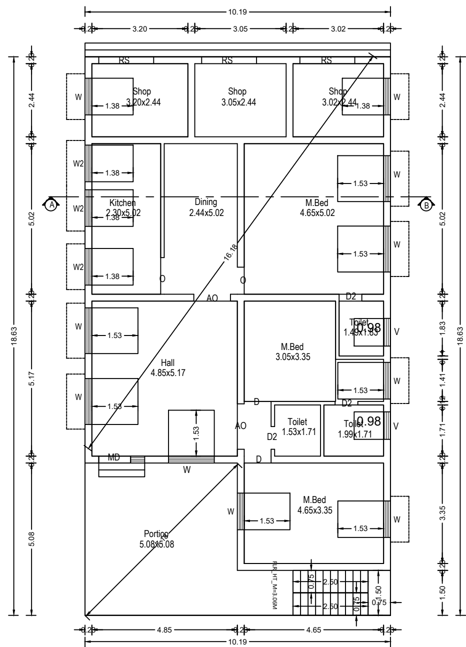
Plan Scale 1:100 Exg. Ground floor
