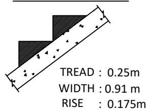
STAIRCASE DETAIL:
