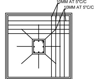
FOOTING DETAIL
