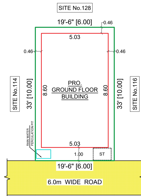
SITE PLAN
