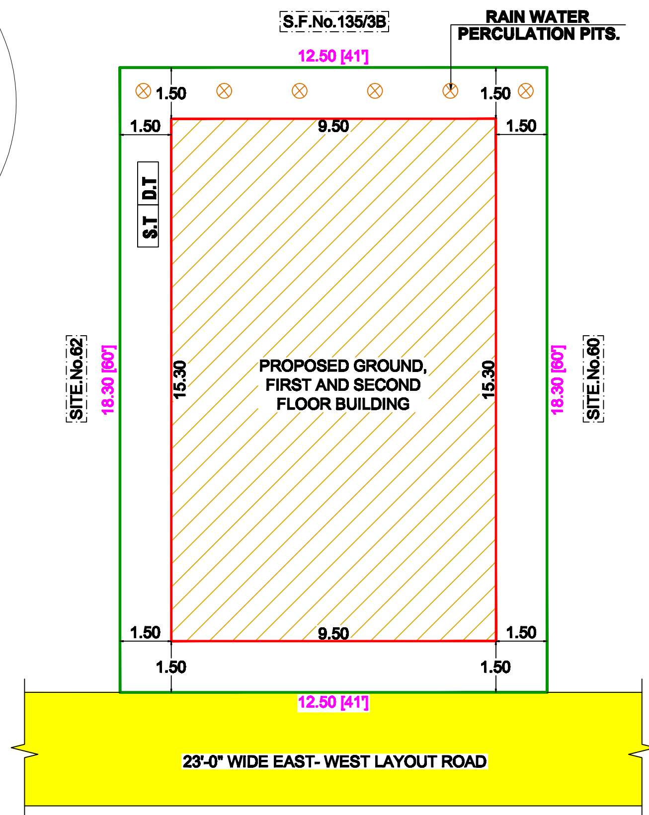
SITE PLAN
