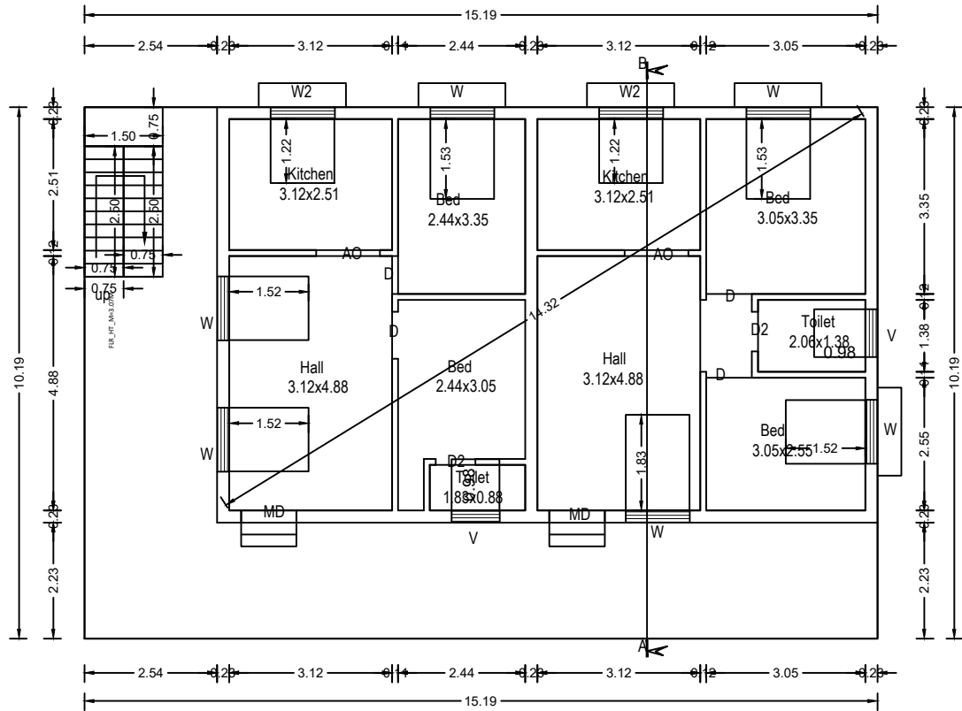
Plan Scale 1:100 Existing Ground floor
