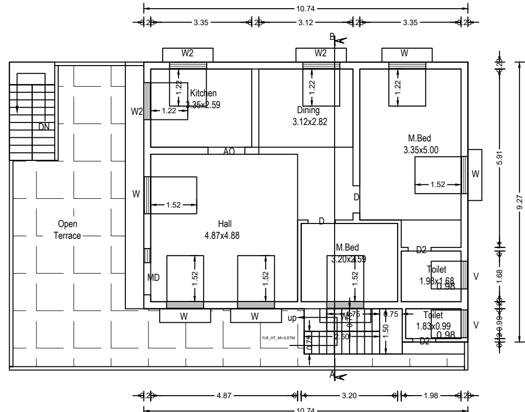
Plan Scale 1:100 Pro .First floor
