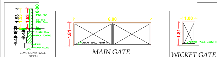
WICKET GATE
