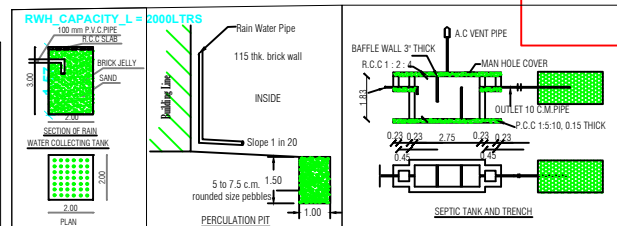
SEPTIC TANK AND TRENCH
