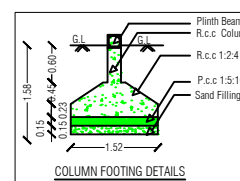
COLUMN FOOTING DETAILS
