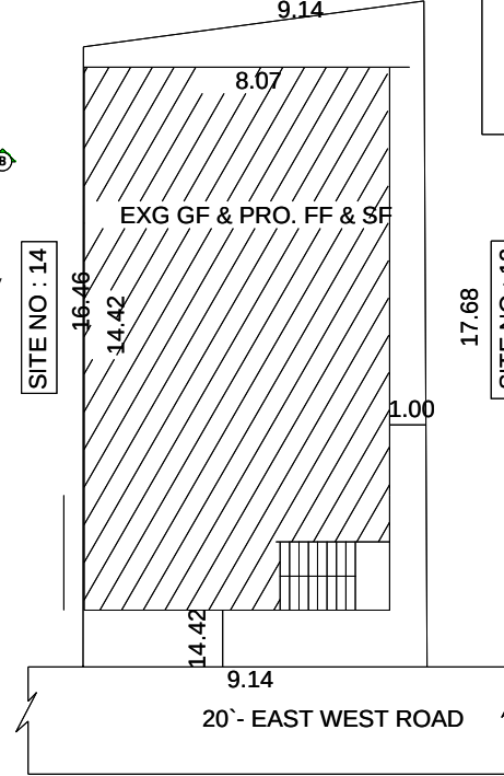
SITE PLAN
