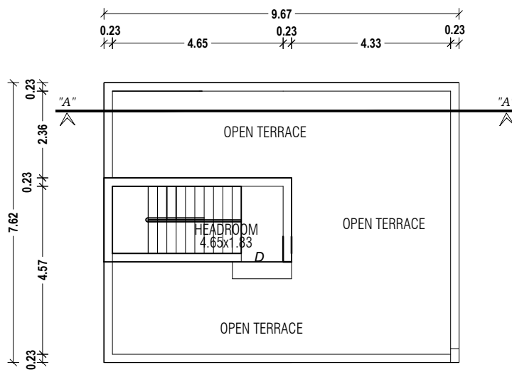
PRO. TERRACE FLOOR PLAN
