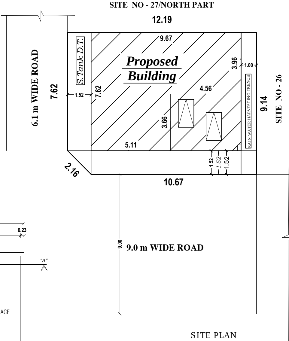
SITE PLAN
