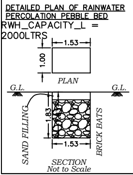
DETAILED PLAN OF RAINWATER PERCOLATION PEBBLE BED
