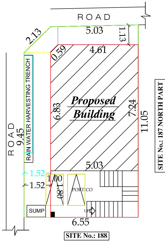
SITE PLAN
