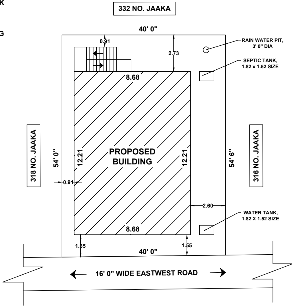
SITE PLAN
