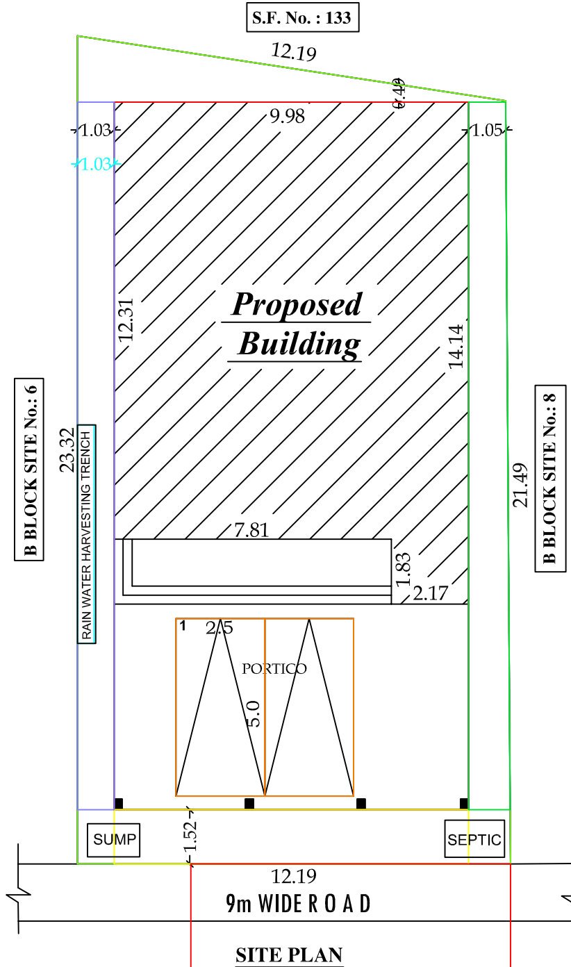
SITE PLAN
