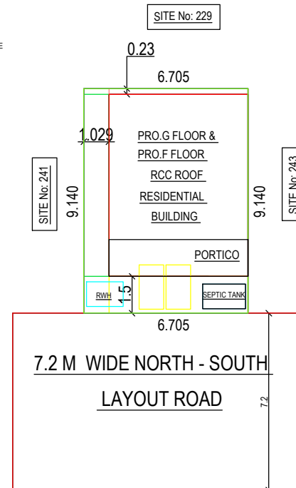
SITE PLAN
