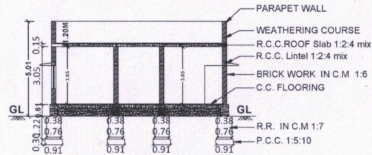
SECTION AT A-A
