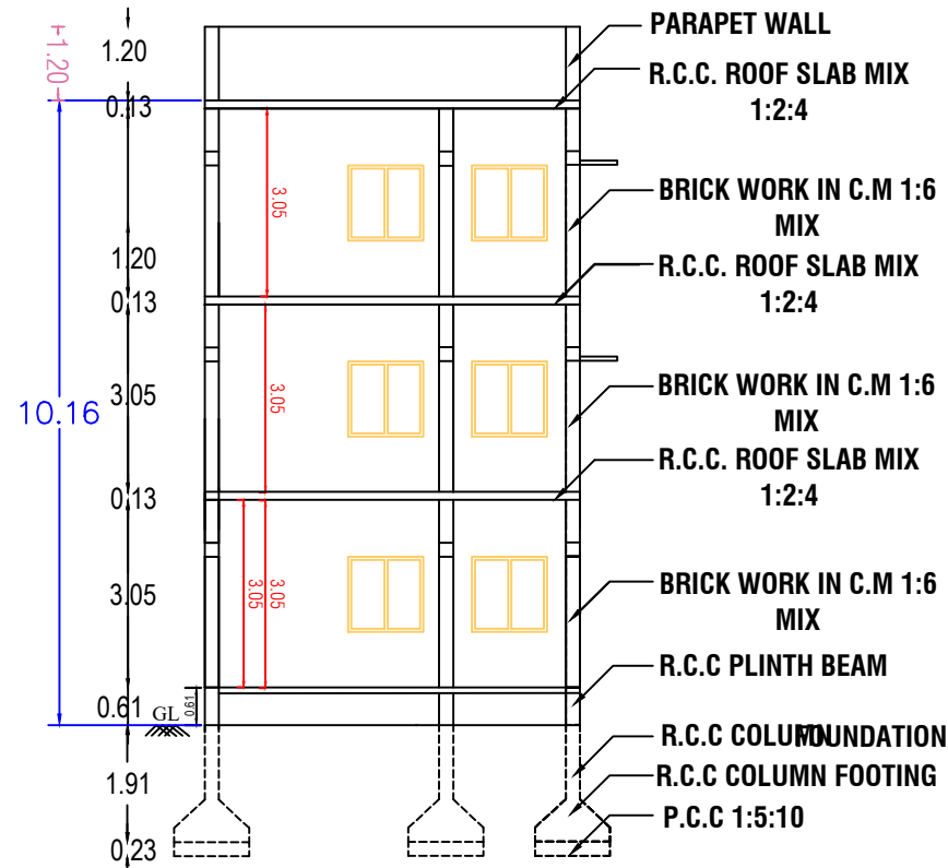
CROSS SECTION AT A-A
