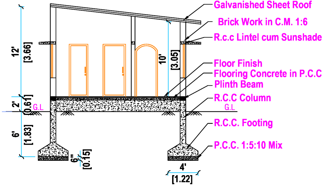
SECTION "AB"
