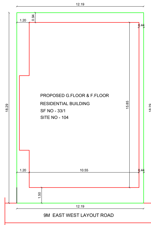
SITE PLAN
