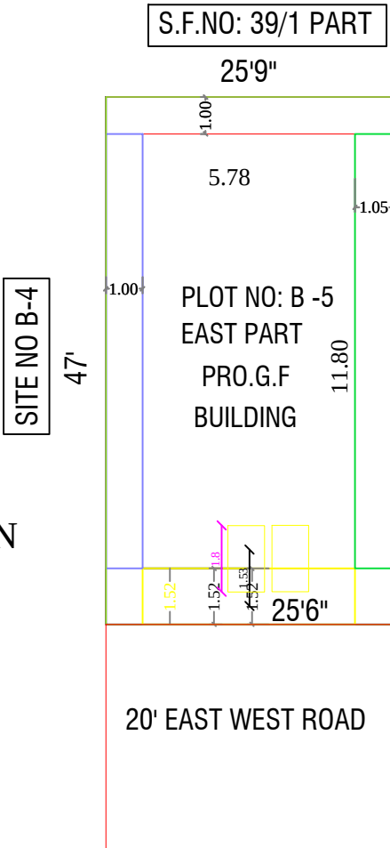
SITE PLAN
