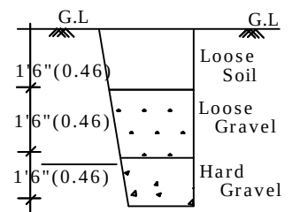
TRIAL PIT (NOT TO SCALE)
