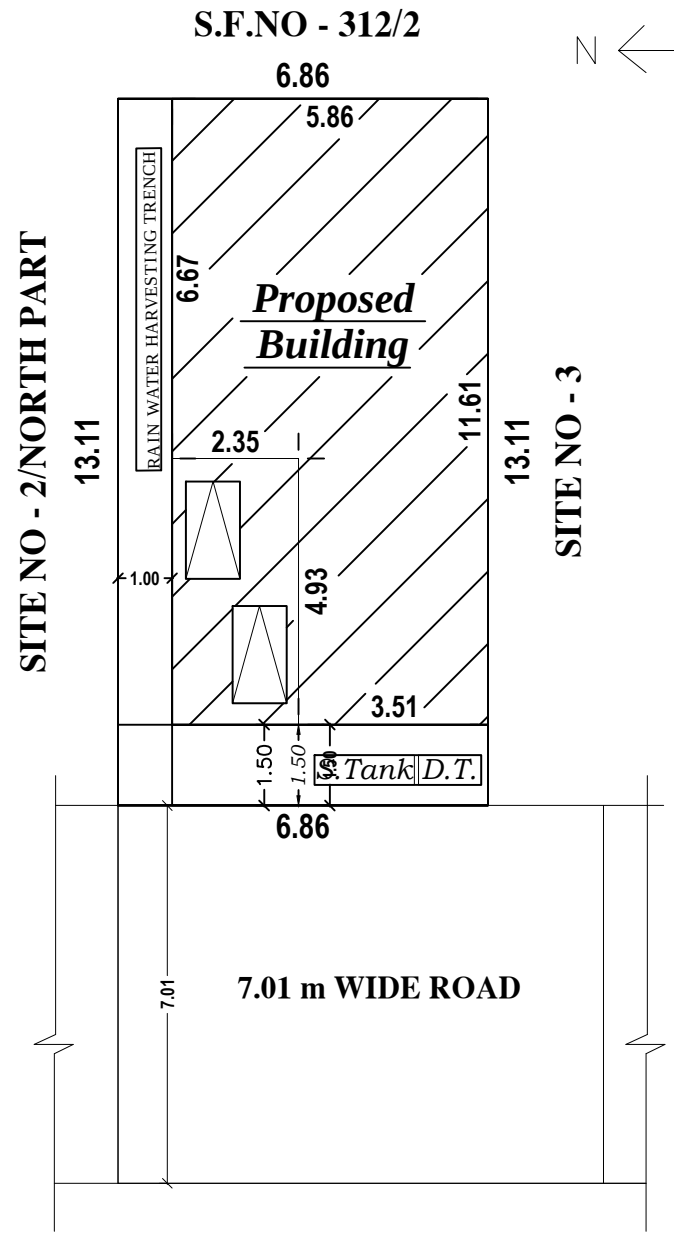
SITE PLAN
