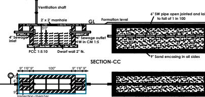
SEPTIC TANK (NTS)
