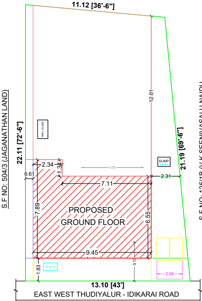
SITE PLAN
