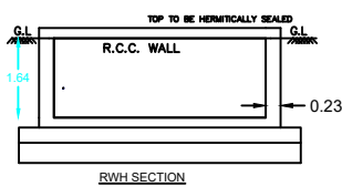
RWH SECTION
