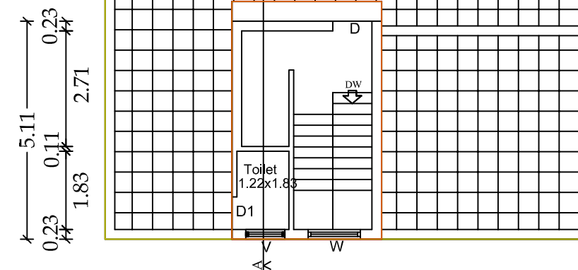
HEAD ROOM PLAN
