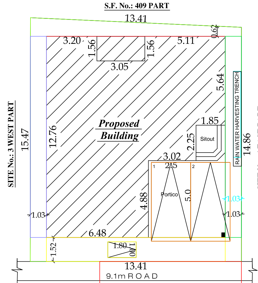
SITE PLAN
