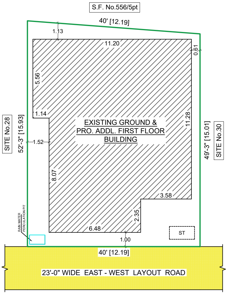
SITE PLAN
