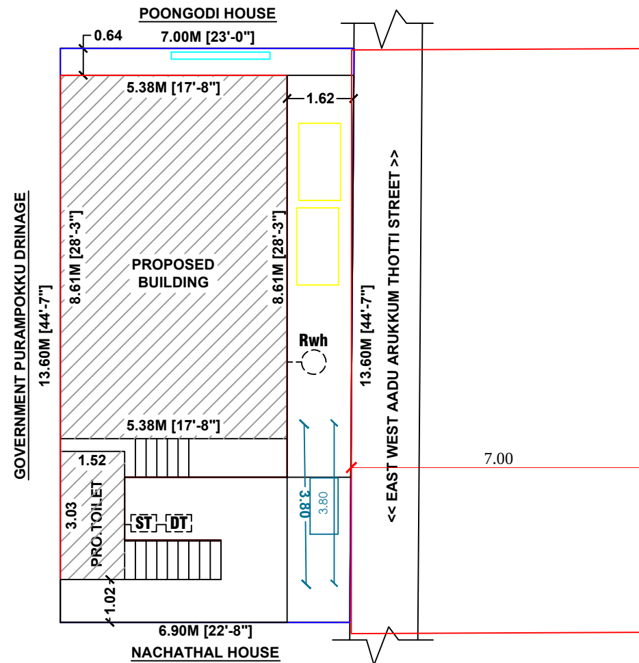
SITE PLAN
