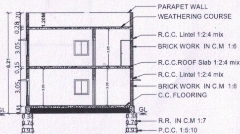
SECTION AT - A A
