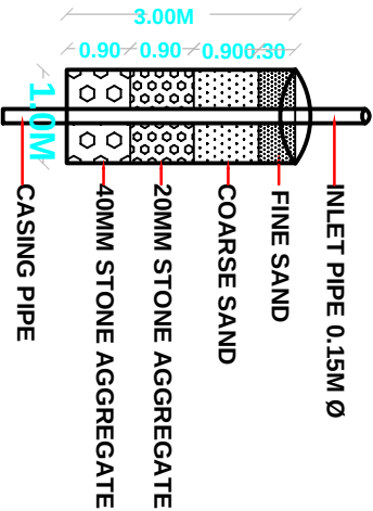
DETAILS OF RAIN WATER
