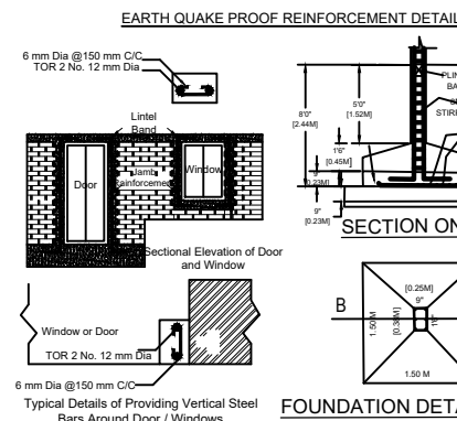
EARTH QUAKE PROOF REINFORCEMENT DETAIL
