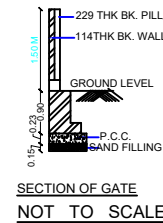
SECTION OF GATE NOT TO SCALE
