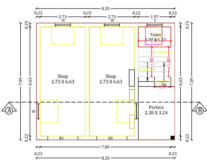
ADDITIONAL AND ALTERATION GROUND FLOOR PLAN
