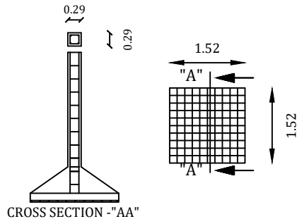
COLUMN DETAILS :-
